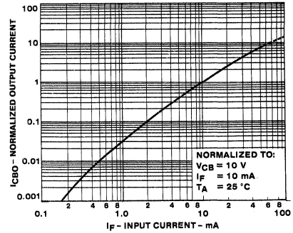
8. OUTPUT CURRENT - COLLECTOR TO BASE VS INPUT CURRENT
