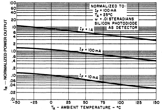
6. OUTPUT VS. TEMPERATURE
