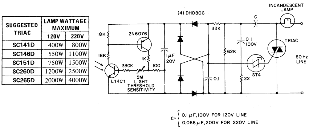
Fig. 79 - Line voltage operated automatic night light.
