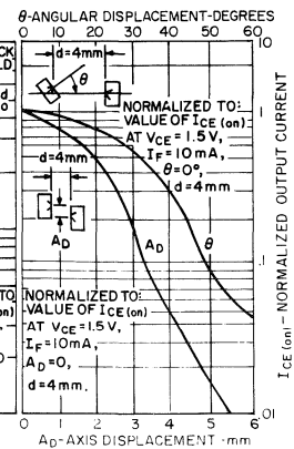
6B. OUTPUT CURRENT VS. DISPLACEMENT (ANGULAR & AXIS)
