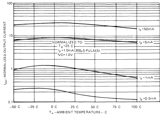
OUTPUT VS. TEMPERATURE
