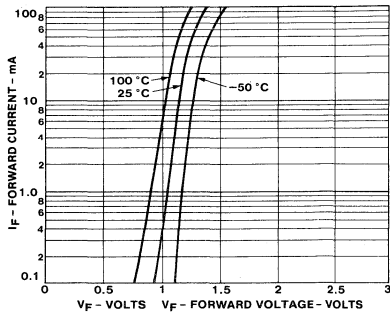
1. INPUT CHARACTERISTICS
