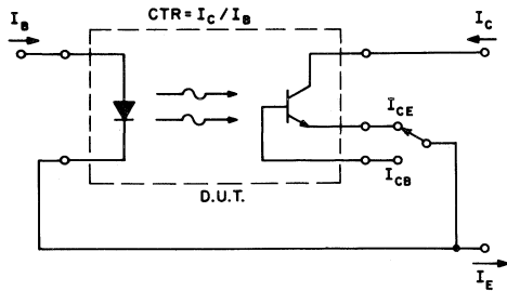
Fig. 74a - CTR tested as transistor h_{FE} .
