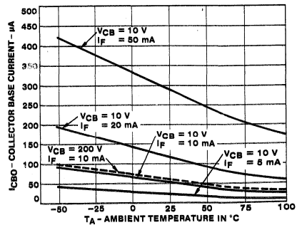
6. COLLECTOR BASE CURRENT VS. TEMPERATURE
