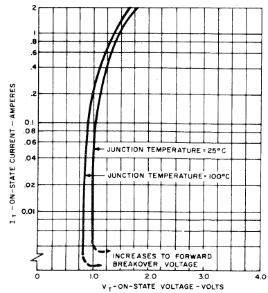
FIGURE 7. ON-STATE CHARACTERISTICS
