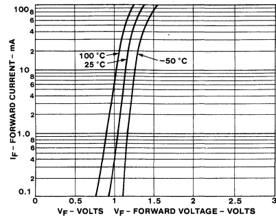
FIGURE 6. INPUT CHARACTERISTICS I F VS. V F
