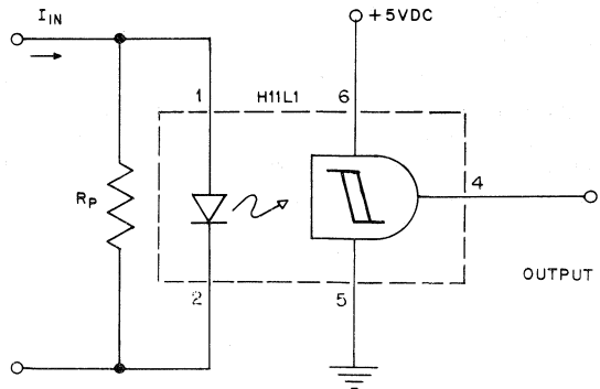
PROGRAMMABLE CURRENT THRESHOLD SENSING CIRCUIT
