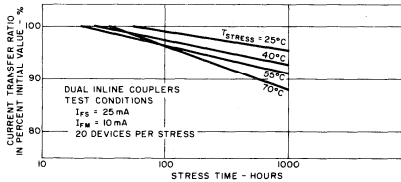
Fig. 64b - Effect of stress temperature on slope.
