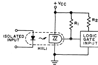
BIAS CIRCUIT FOR TTL, HNIL, CMOS, I 2 L, NMOS AND PMOS
