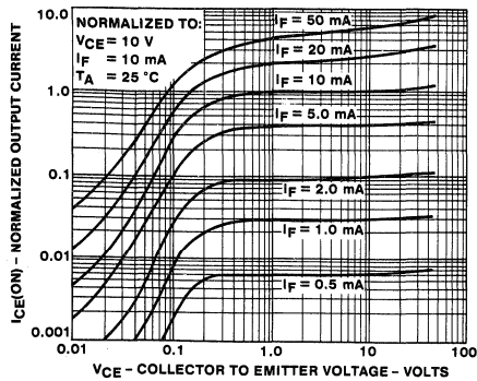
5. OUTPUT CHARACTERISTICS
