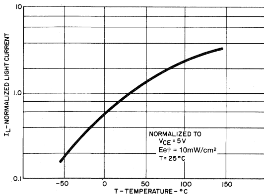
NORMALIZED LIGHT CURRENT VS TEMPERATURE
