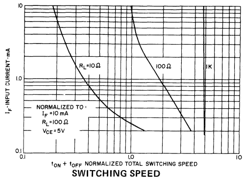
SWITCHING SPEED
