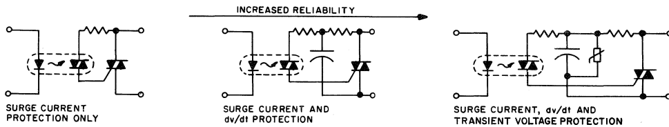
Fig. 52 - Elimination of triac driver malfunction and failure.
