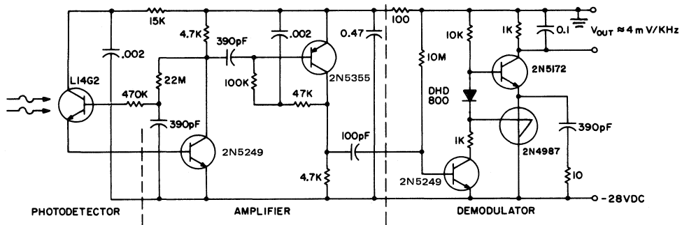
Fig. 97 - Receiver for 50kHz FM optical transmitter.
