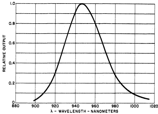
5. SPECTRAL OUTPUT
