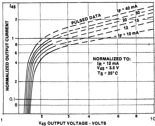
1. OUTPUT CHARACTERISTICS
