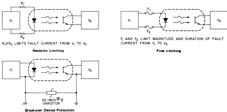
Fig. 31 - Methods of limiting or eliminating dielectric breaker problems.
