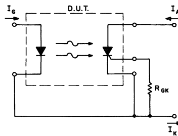
Fig. 74b - I_{FT} tested as SCR I_{Gt} .
