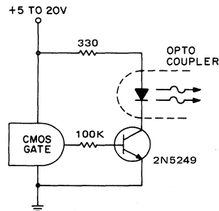
Fig. 120b - NPN buffered CMOS connection I_o \geq 7\text{mA} .
