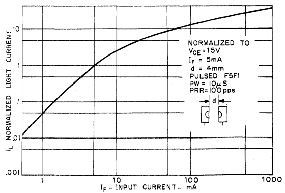
6. COUPLED LIGHT CURRENT VS. F5F1 INPUT CURRENT
