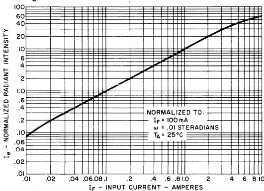
1. RADIANT INTENSITY VS. INPUT CURRENT \Delta I_e/\Delta I_f
