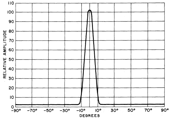
4. ANGULAR RESPONSE
