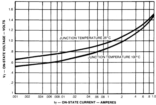
9. ON-STATE CHARACTERISTICS
