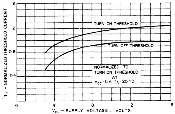
THRESHOLD CURRENT VS. SUPPLY VOLTAGE
