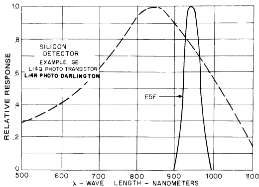
5. SPECTRAL RESPONSE
