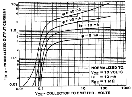
4. OUTPUT CHARACTERISTICS
