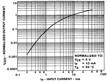
OUTPUT CURRENT VS INPUT CURRENT
