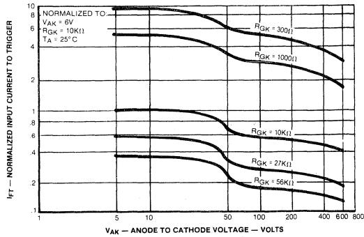
1. INPUT CURRENT TO TRIGGER VS. ANODE TO CATHODE VOLTAGE
