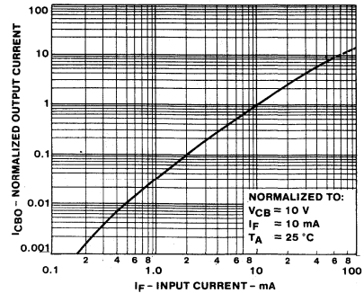
6. OUTPUT CURRENT ( I_{CBO} ) VS INPUT CURRENT
