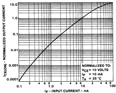
4. OUTPUT CURRENT VS INPUT CURRENT
