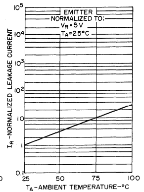
6. LEAKAGE CURRENTS VS. TEMPERATURE
