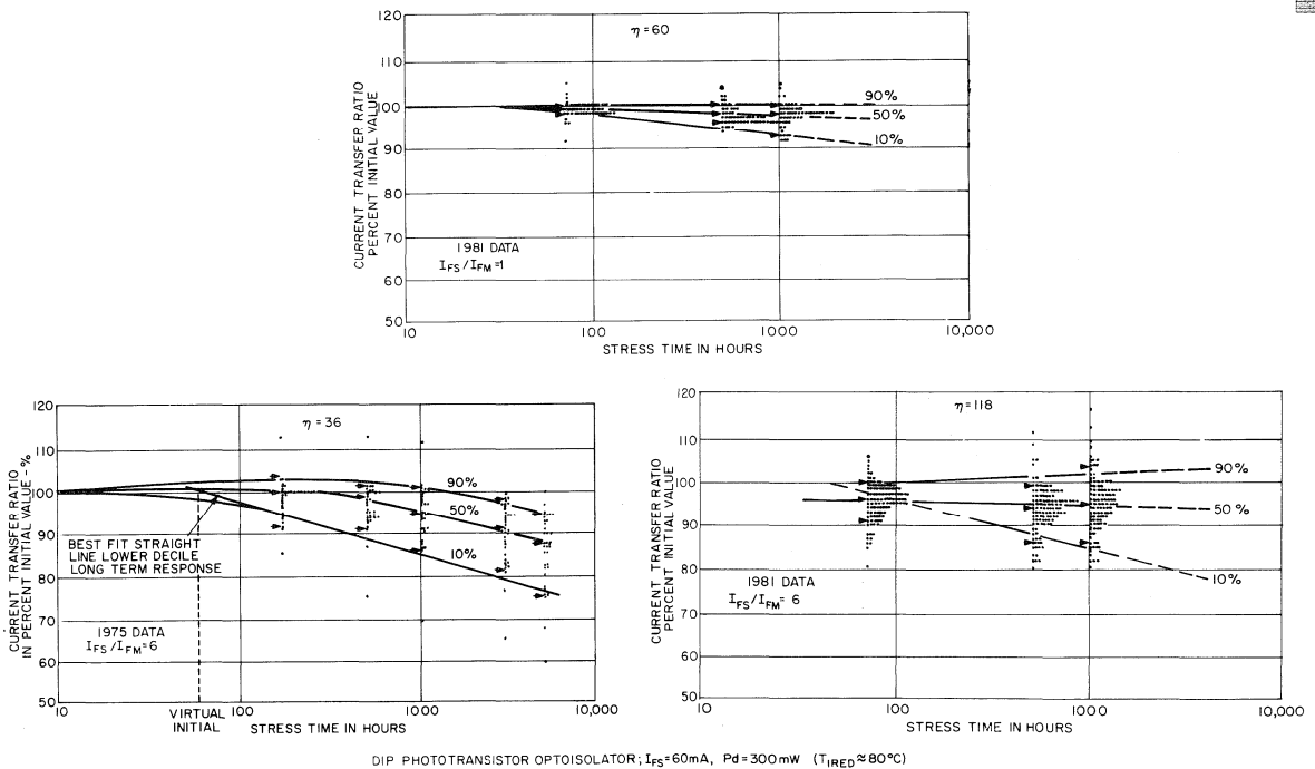
Fig. 62 - Life test results — illustrating observed change in IRED output with operating time.
