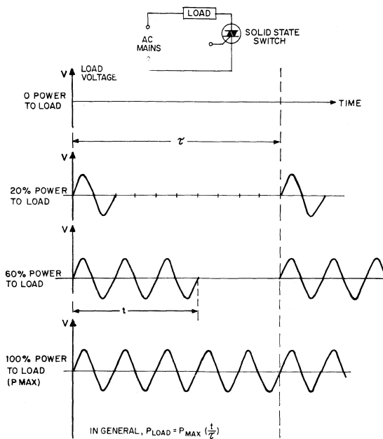
Fig. 158 - Principle of zero voltage switching.
