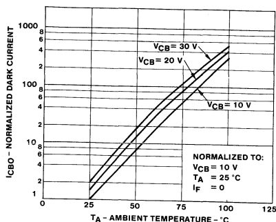
4. I_{CBO} VS. TEMPERATURE
