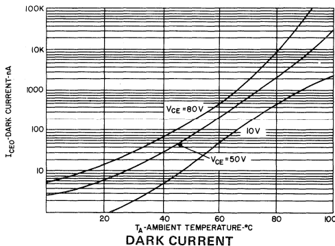
DARK CURRENT
