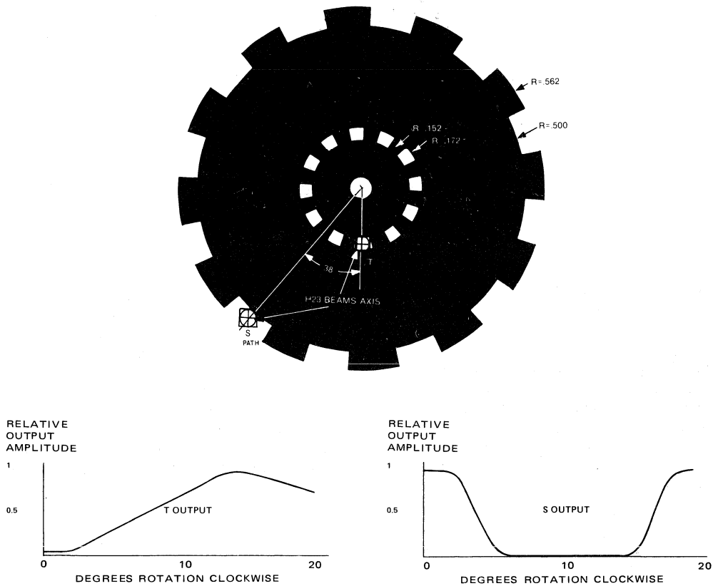
Fig. 28 - Cost optimized shaft encoder.
