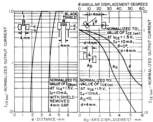
6A. OUTPUT CURRENT VS. SHIELD DISTANCE
