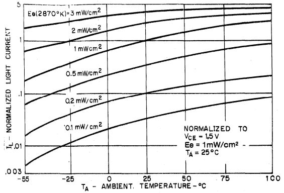
2. LIGHT CURRENT VS. AMBIENT TEMPERATURE
