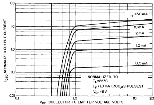
OUTPUT CHARACTERISTICS
