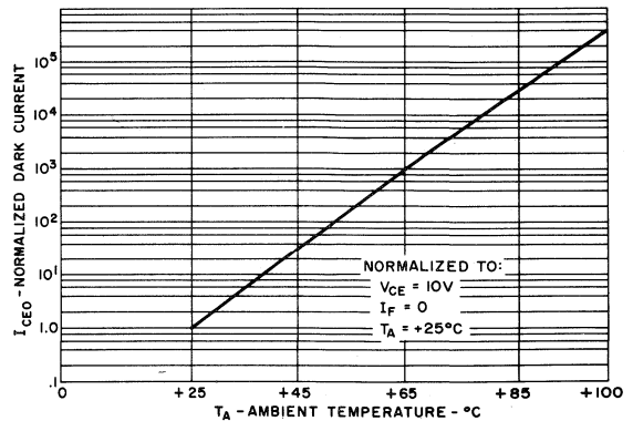
NORMALIZED DARK CURRENT VS TEMPERATURE
