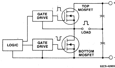
Fig. 7 - Half-bridge power-MOSFET circuit.
