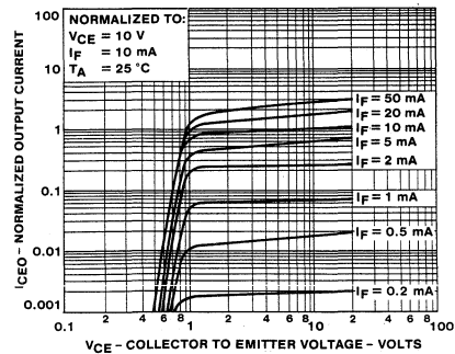
4. OUTPUT CHARACTERISTICS
