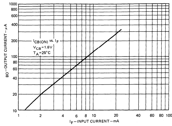
OUTPUT CURRENT — COLLECTOR-BASE VS. INPUT CURRENT
