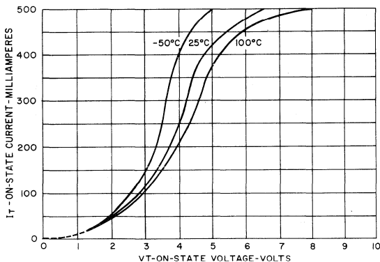
FIGURE 3. ON-STATE VOLTAGE VS. OUTPUT CURRENT
