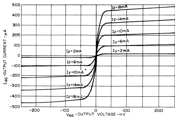
3. OUTPUT CHARACTERISTICS
