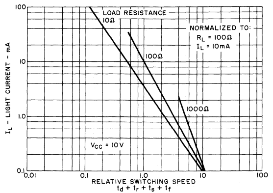
6. LIGHT CURRENT VS. RELATIVE SWITCHING SPEED
