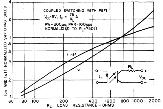
4. SWITCHING TIME VS. LOAD RESISTANCE
