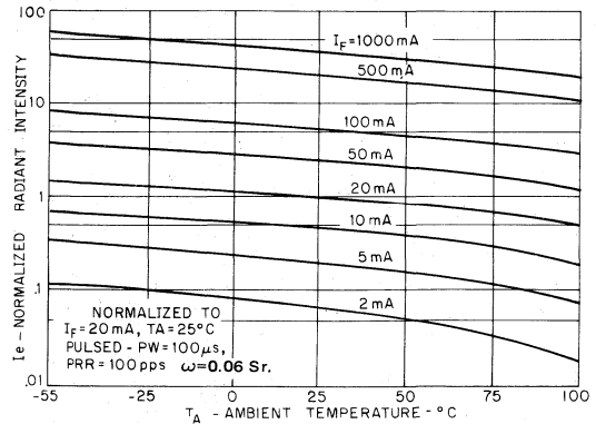
2. RADIANT INTENSITY VS. TEMPERATURE
