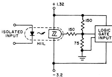
Fig. 57 - H11L input for ECL logic.
