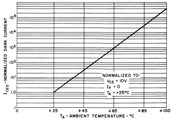
6. NORMALIZED DARK CURRENT VS TEMPERATURE
