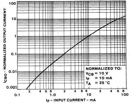
8. OUTPUT CURRENT — COLLECTOR-TO-BASE VS. INPUT CURRENT
