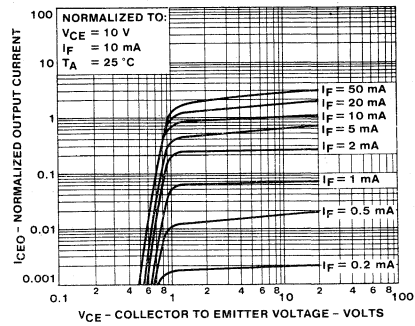
4. OUTPUT CHARACTERISTICS
