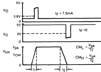
TEST CIRCUIT AND VOLTAGE WAVEFORMS
