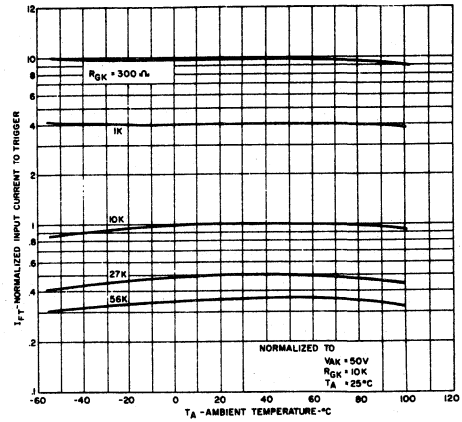
FIGURE 2. INPUT CURRENT TO TRIGGER VS. TEMPERATURE
