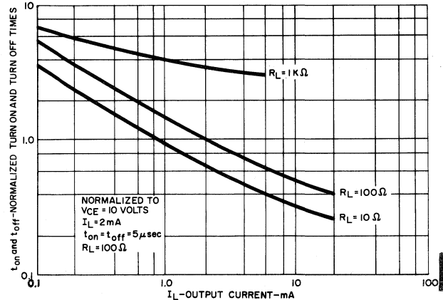
SWITCHING TIMES VS OUTPUT CURRENT
