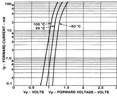
1. INPUT CHARACTERISTICS
