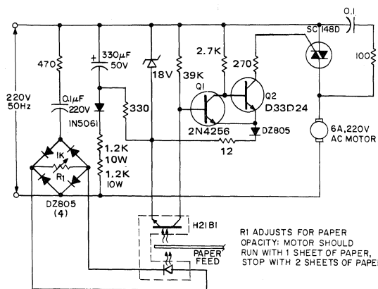
Fig. 88 - Paper sheet discriminator with zero voltage switching triac motor drive.
