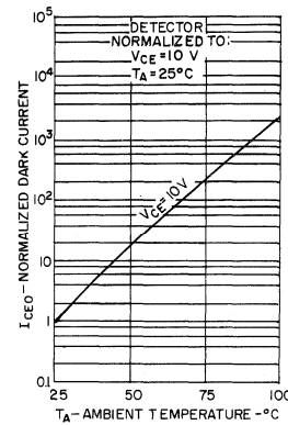
6. LEAKAGE CURRENTS VS. TEMPERATURE
