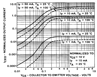
6. OUTPUT CHARACTERISTICS
