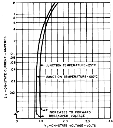
FIGURE 12. ON-STATE CHARACTERISTICS
