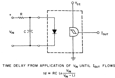
Fig. 35 - Time delay operation of optocoupler.
