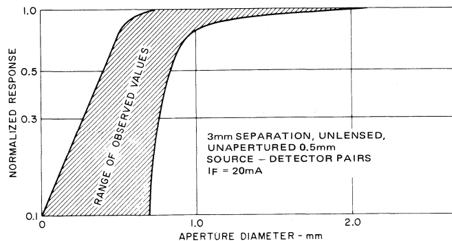
Fig. 25 - Effect of aperture size on response transparent aperture on opaque field.
