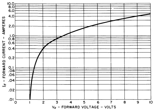
3. FORWARD VOLTAGE VS. FORWARD CURRENT
