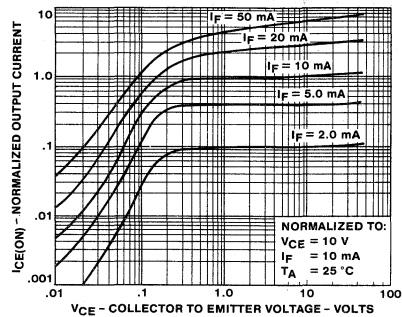
OUTPUT CHARACTERISTICS
