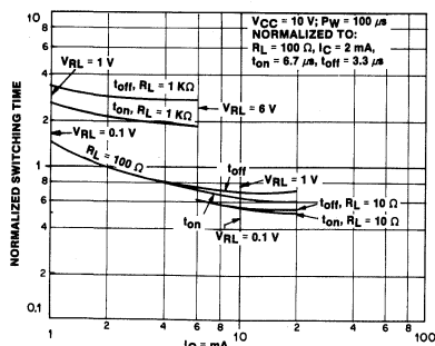
SWITCHING SPEED VS. COLLECTOR CURRENT (NOT SATURATED)
