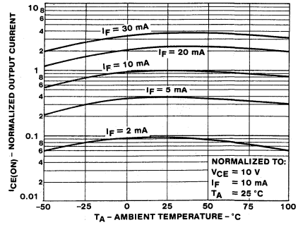
2. OUTPUT CURRENT VS TEMPERATURE
