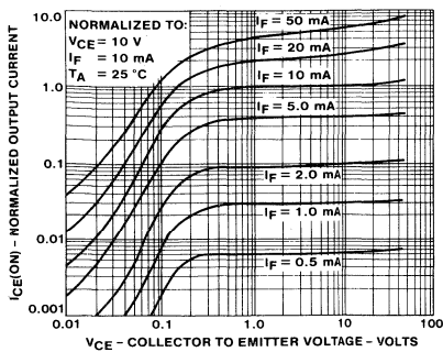
5. OUTPUT CHARACTERISTICS
