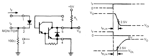
SWITCHING TEST CIRCUIT
