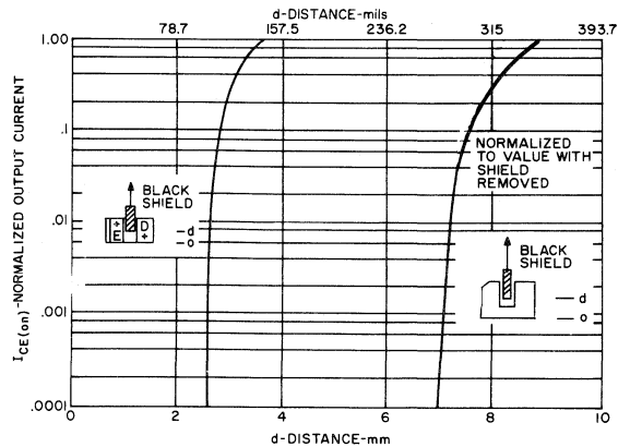
6. OUTPUT CURRENT VS. SHIELD DISTANCE
