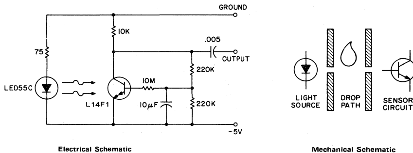
Fig. 90 - Low light level drop detector.
