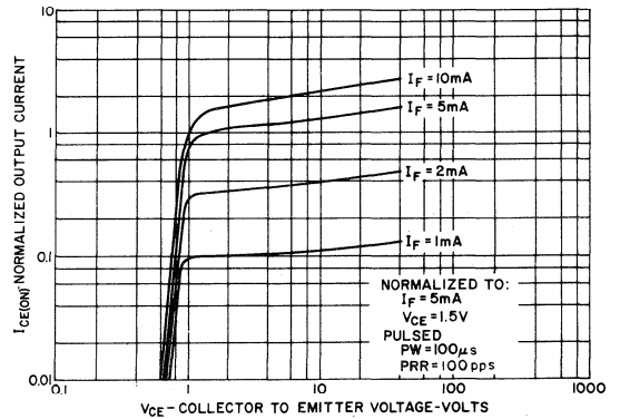
4. OUTPUT CHARACTERISTICS
