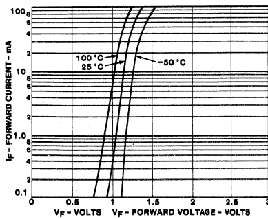
7. FORWARD VOLTAGE VS. FORWARD CURRENT
