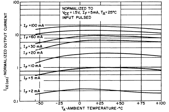
2. OUTPUT CURRENT VS. TEMPERATURE
