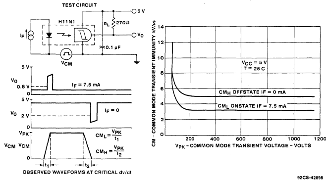
Fig. 3 - H11N common-noise transient immunity.
