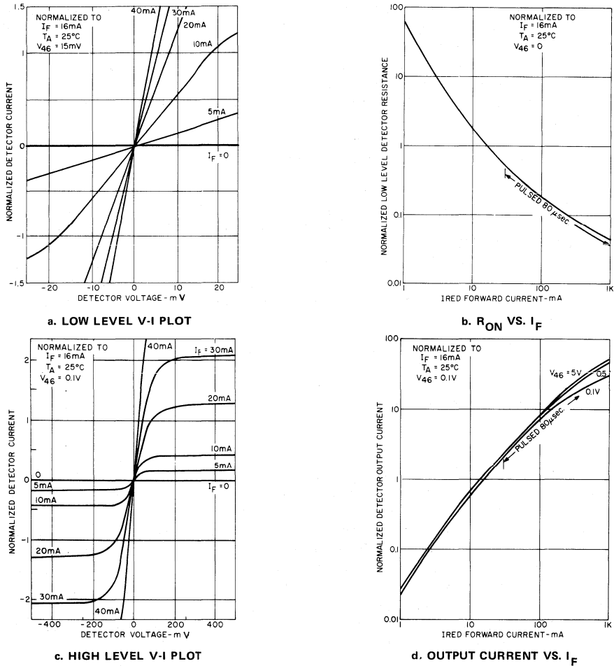
Fig. 49 - Bilateral analog FET characteristics.
