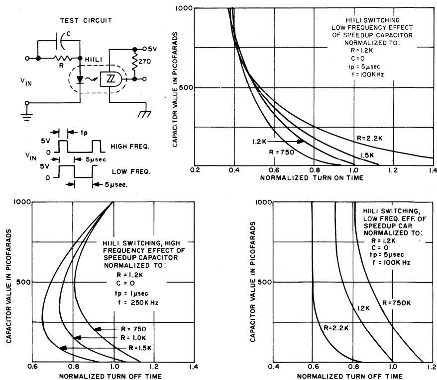
Fig. 55 - H11L switching.
