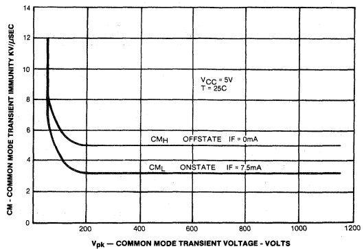
CM L AND CM H VS COMMON MODE TRANSIENT VOLTAGE
