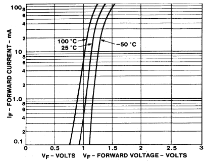
INPUT CHARACTERISTICS
