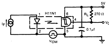
TEST CIRCUIT AND VOLTAGE WAVEFORMS
