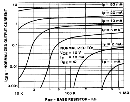
10. OUTPUT CURRENT VS. BASE EMITTER RESISTANCE
