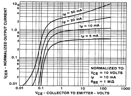
4. OUTPUT CHARACTERISTICS
