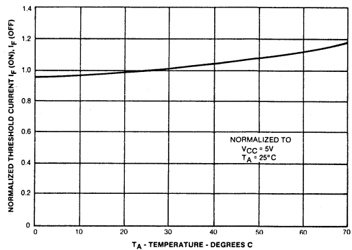
THRESHOLD CURRENT VS TEMPERATURE
