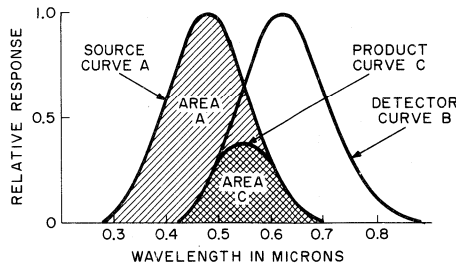
Fig. 16 - Effectiveness of Source A on Detector B.
