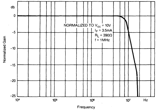
H11V GAIN ROLLOFF
