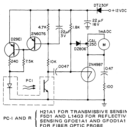
Fig. 89 - Optical pickup tachometer.
