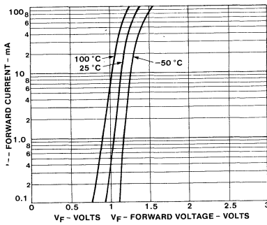
INPUT CHARACTERISTICS
