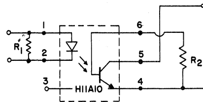
THRESHOLD SWITCH BIAS CIRCUIT ILLUSTRATION
