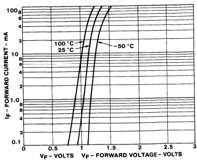
1. INPUT CHARACTERISTICS
