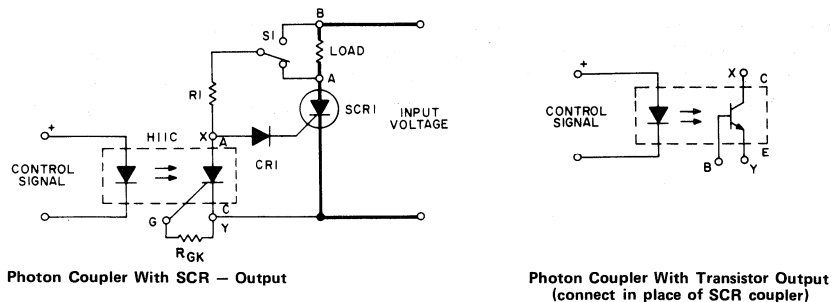
Fig. 138 - Normally closed configurations.
