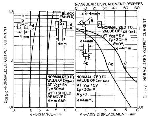
6B. OUTPUT CURRENT VS. DISPLACEMENT (ANGULAR & AXIS)
