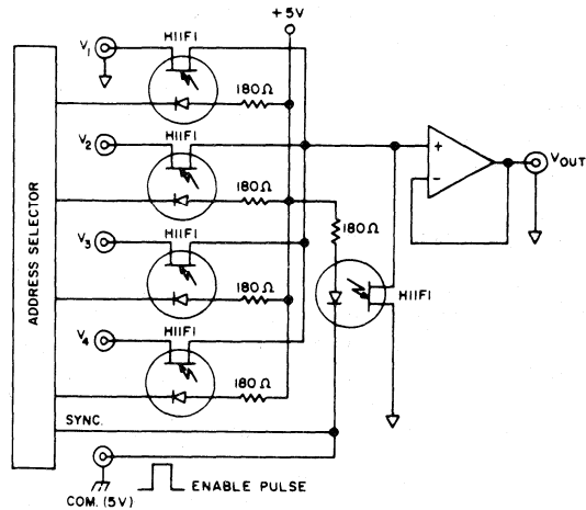
Fig. 116 - Four channel multiplexer.
