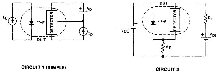
Fig. 68 - Burn-in circuit configurations.
