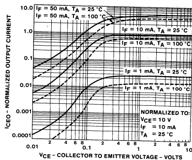
6. OUTPUT CHARACTERISTICS
