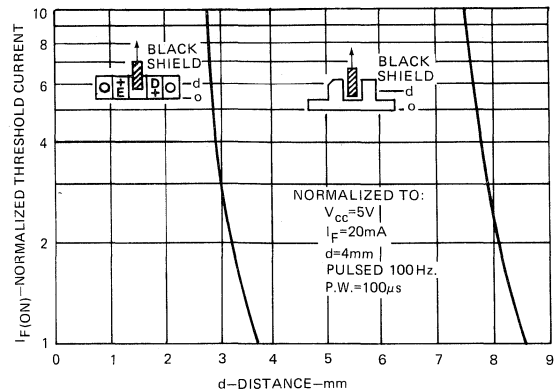
THRESHOLD CURRENT VS. SHIELD DISTANCE
