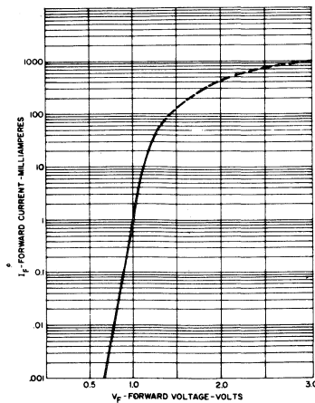
FIGURE 6. INPUT CHARACTERISTICS I F VS. V F
