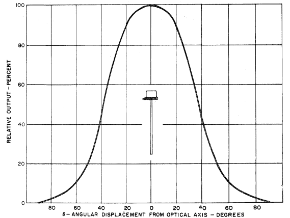
6. CQX15-CQX17 TYPICAL RADIATION PATTERN
