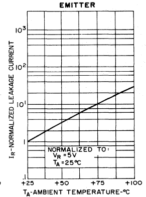
4. LEAKAGE CURRENTS VS. TEMPERATURE
