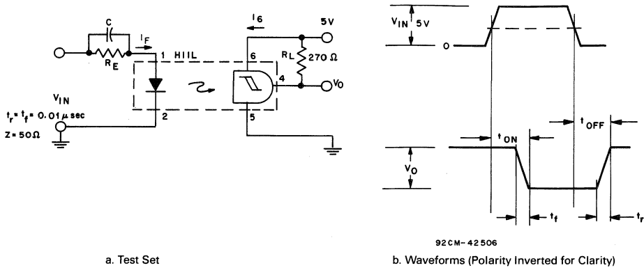
Fig. 75 - Switching time testing.
