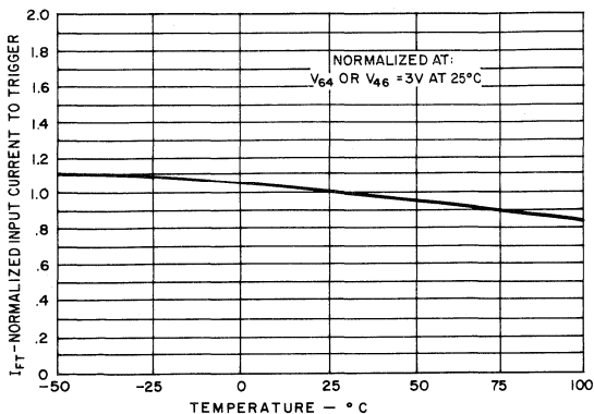
FIGURE 1. INPUT CURRENT TO TRIGGER VS. TEMPERATURE
