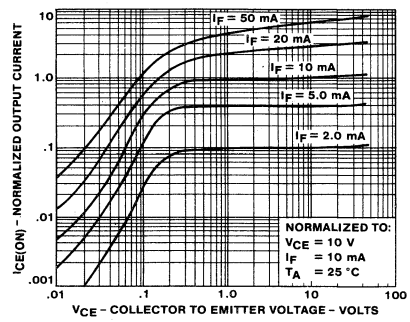
OUTPUT CHARACTERISTICS
