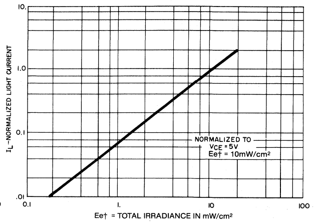
NORMALIZED LIGHT CURRENT VS RADIATION
