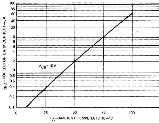
I CBO VS. TEMPERATURE
