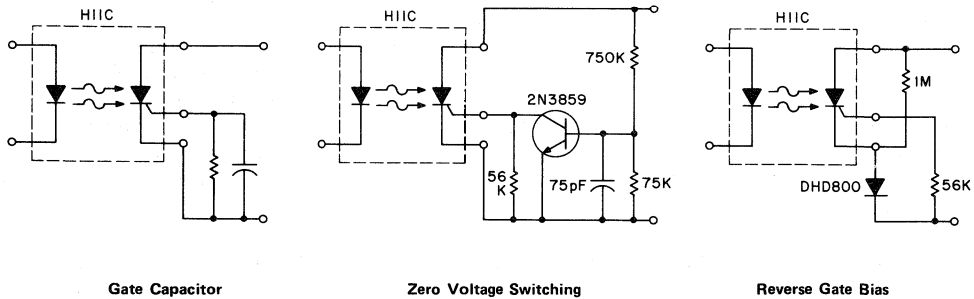
Fig. 48 - Methods used to optimize R_{GK} effect.
