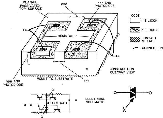
Fig. 51 - Simple triac driver concept.
