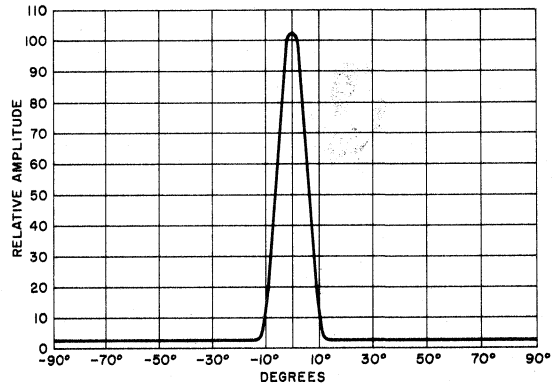
4. ANGULAR RESPONSE
