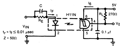
SWITCHING TEST CIRCUIT
