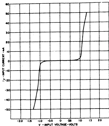
1. INPUT CHARACTERISTICS
