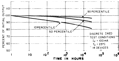
Fig. 63 - Long-term IRED life test results.
