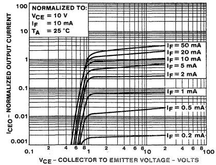
4. OUTPUT CHARACTERISTICS
