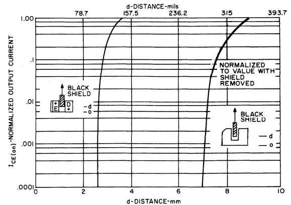
6. OUTPUT CURRENT VS. SHIELD DISTANCE
