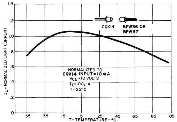
NORMALIZED LIGHT CURRENT VS TEMPERATURE
