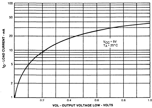
ON VOLTAGE VS LOAD CURRENT
