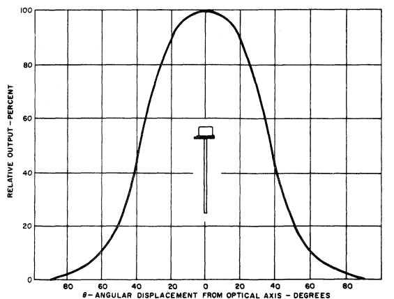
6. 1N6265 - TYPICAL RADIATION PATTERN
