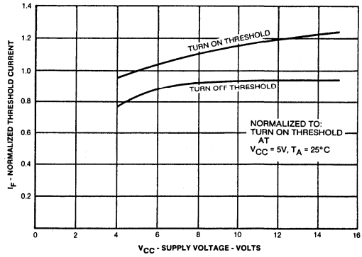
THRESHOLD CURRENT VS SUPPLY VOLTAGE
