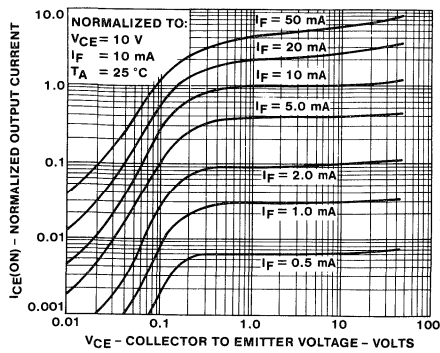
5. OUTPUT CHARACTERISTICS
