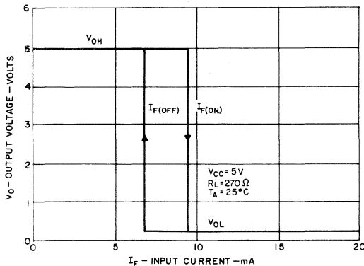
1. TRANSFER CHARACTERISTICS
