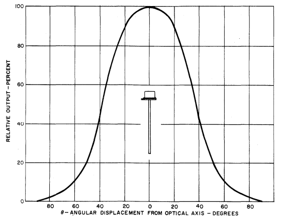
6. LED 55BF, 55CF, 56F TYPICAL RADIATION PATTERN
