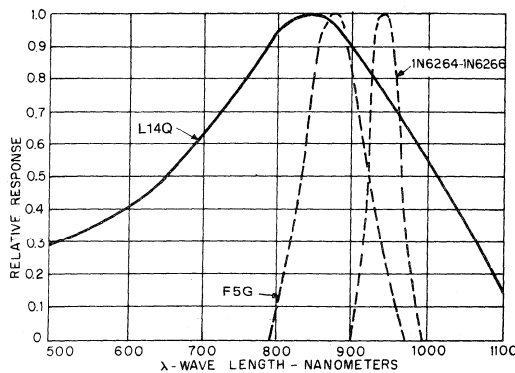
5. SPECTRAL RESPONSE
