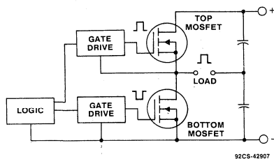
Fig. 1 - Half-bridge power-MOSFET circuit.
