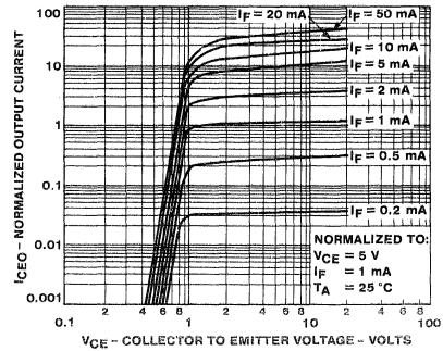
OUTPUT CHARACTERISTICS
