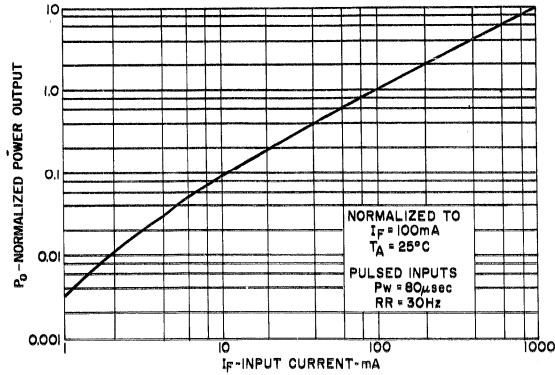
1. POWER OUTPUT VS. INPUT CURRENT
