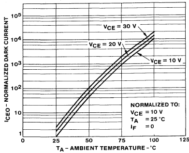
3. DARK I_{CO} CURRENT VS TEMPERATURE
