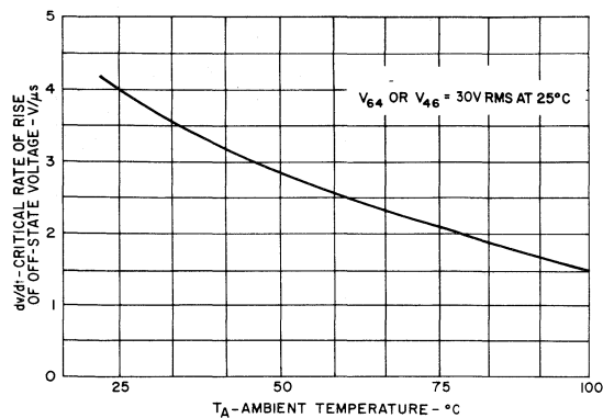
FIGURE 5. dv/dt VS. TEMPERATURE
