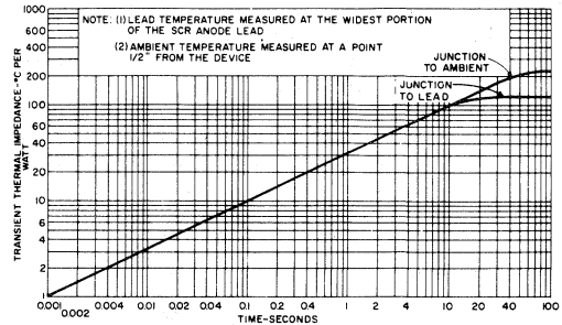
FIGURE 3. MAXIMUM TRANSIENT THERMAL IMPEDANCE
