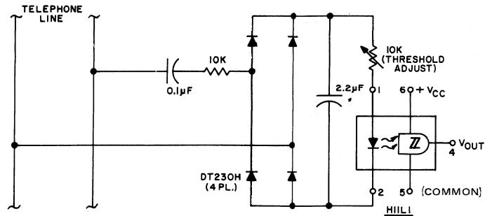
Fig. 109 - Ring detector using H11L1.
