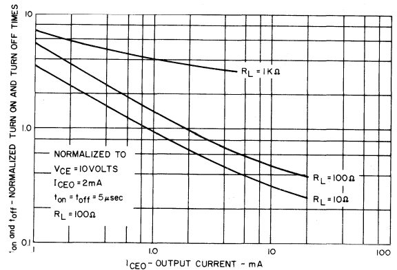
SWITCHING TIMES VS OUTPUT CURRENT
