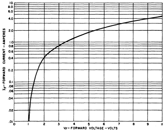
3. FORWARD VOLTAGE VS. FORWARD CURRENT
