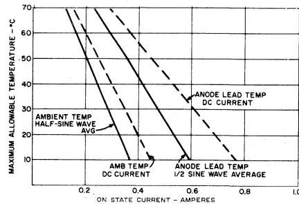
FIGURE 5. ON-STATE CURRENT VS. MAXIMUM ALLOWABLE TEMPERATURE
