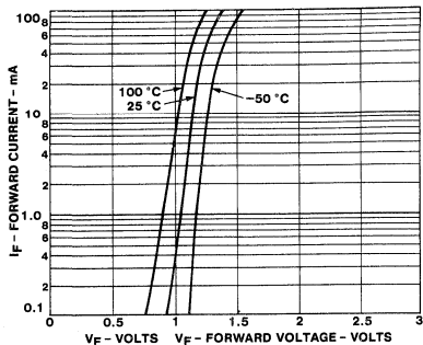
2. INPUT CHARACTERISTICS
