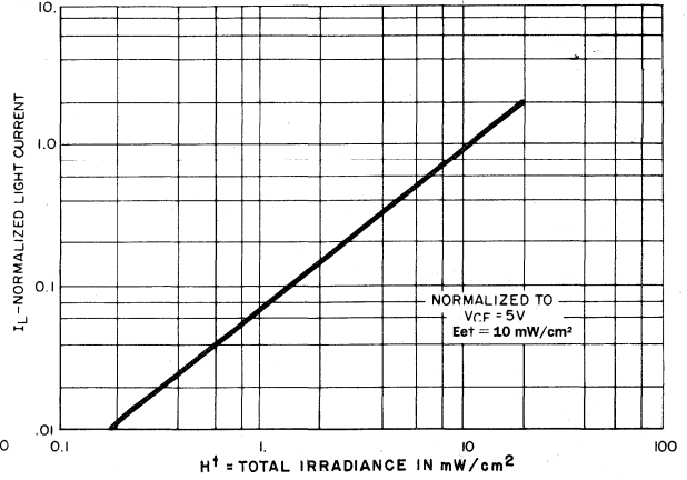
NORMALIZED LIGHT CURRENT VS RADIATION
