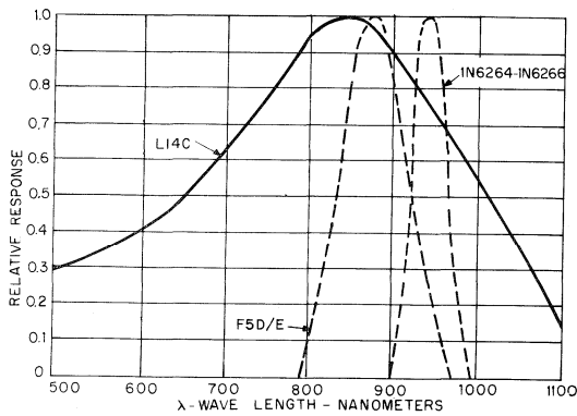
SPECTRAL RESPONSE
