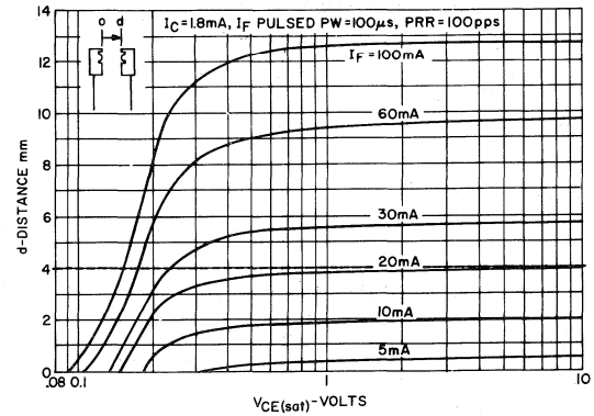
4. V_{CE(sat)} VS. DISTANCE
