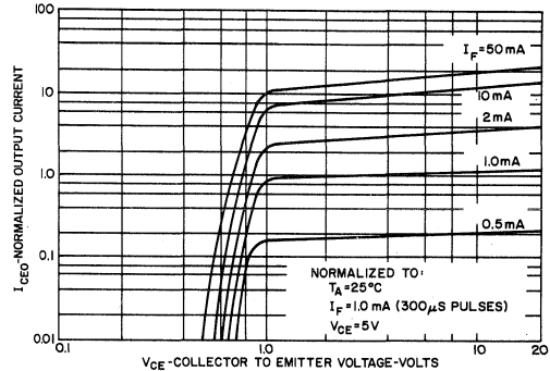
OUTPUT CHARACTERISTICS
