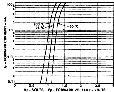
FIGURE 6. INPUT CHARACTERISTICS I F VS. V F
