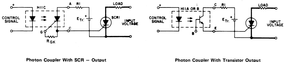
Fig. 137 - Photon coupler triggering main SCR 1 using separate power supply.
