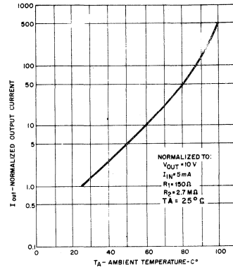
4. LEAKAGE
