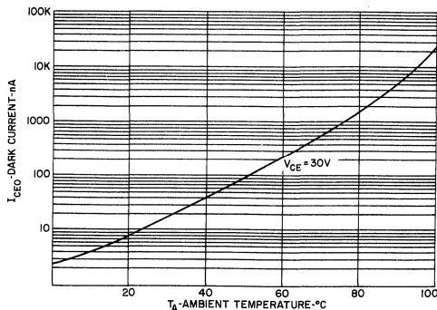
DARK CURRENT
