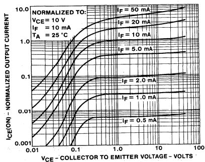
5. OUTPUT CHARACTERISTICS
