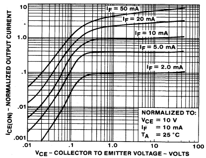
OUTPUT CHARACTERISTICS
