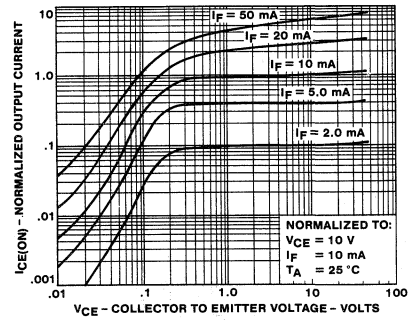
4. OUTPUT CHARACTERISTICS
