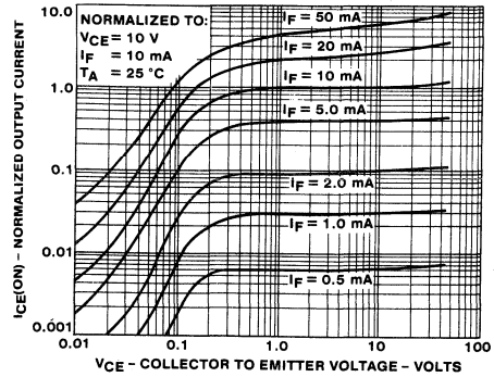
8. OUTPUT CHARACTERISTICS
