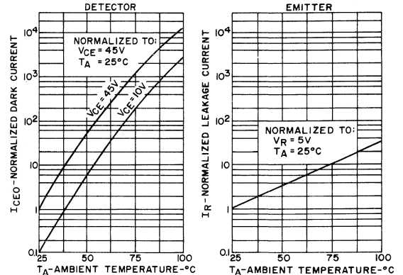
4. LEAKAGE CURRENTS VS. TEMPERATURE
