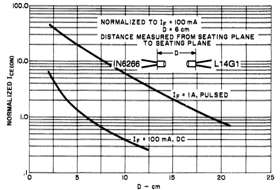
8. IL VS. DISTANCE IRED/PHOTOTRANSISTOR PAIR
