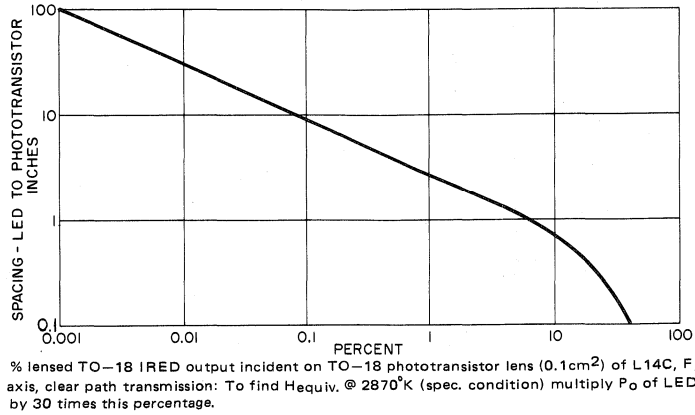
Fig. 18 - Lensed LED to phototransistor coupling chart.
